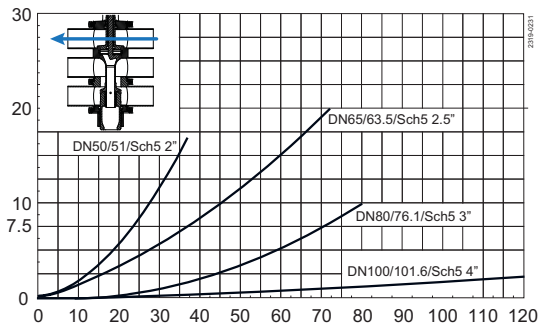
Fig. 3. Pressure drop/capacity diagram, upper body.
