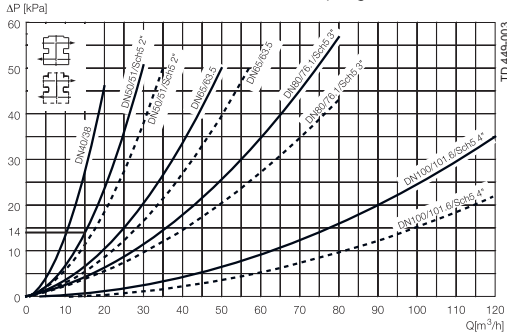
Fig. 5. Pressure drop/capacity diagram, between bodies.
