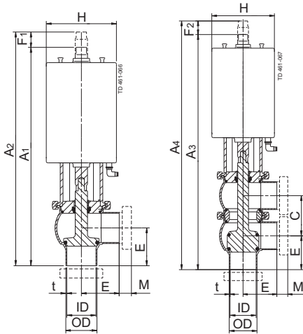
Shut-off valve
